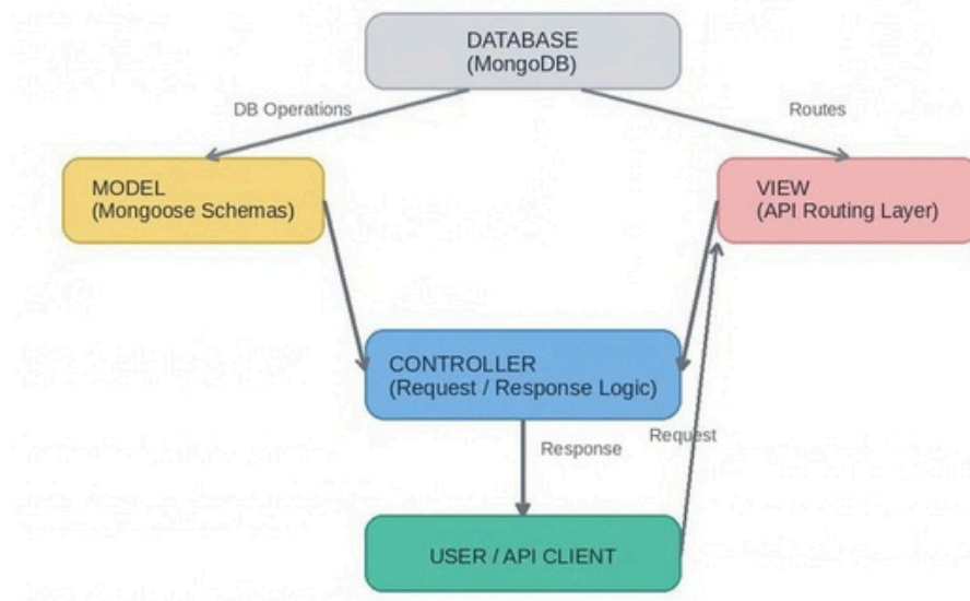
Figure 11.1: MVC Architecture Pattern for AI WeatherWise
